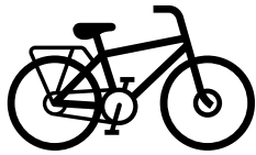
Bicycle
