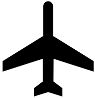
Airplane
