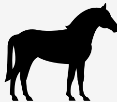
Horse
